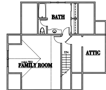
UPPER LEVEL FLOOR PLAN
