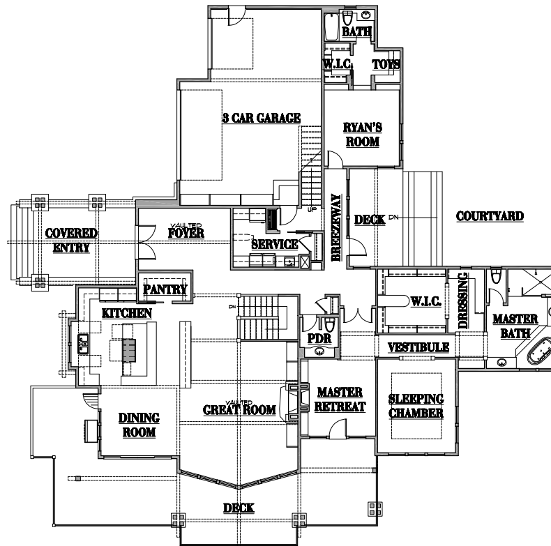
MAIN LEVEL FLOOR PLAN
